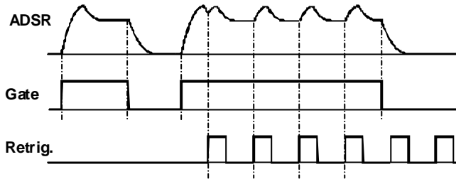
Fig. 2: Envelope re-trigger system
