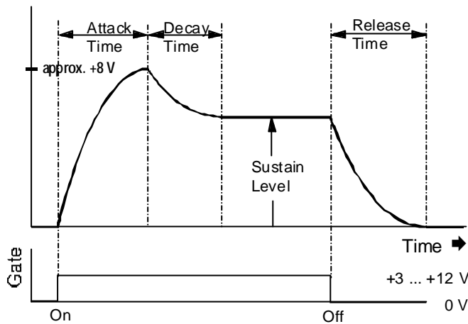
Fig. 1: An ADSR envelope and its parameters
